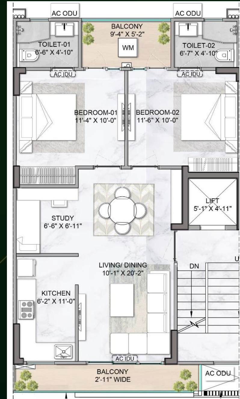
TYPICAL FLOOR
